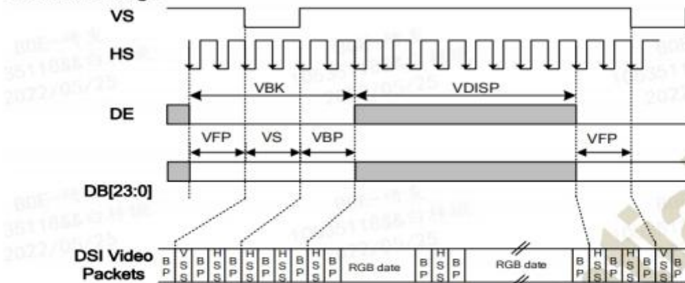
Vertical Timings
