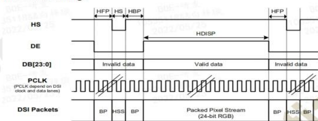
Horizontal Timings
